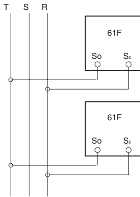
Fig. 2 Match Phases
